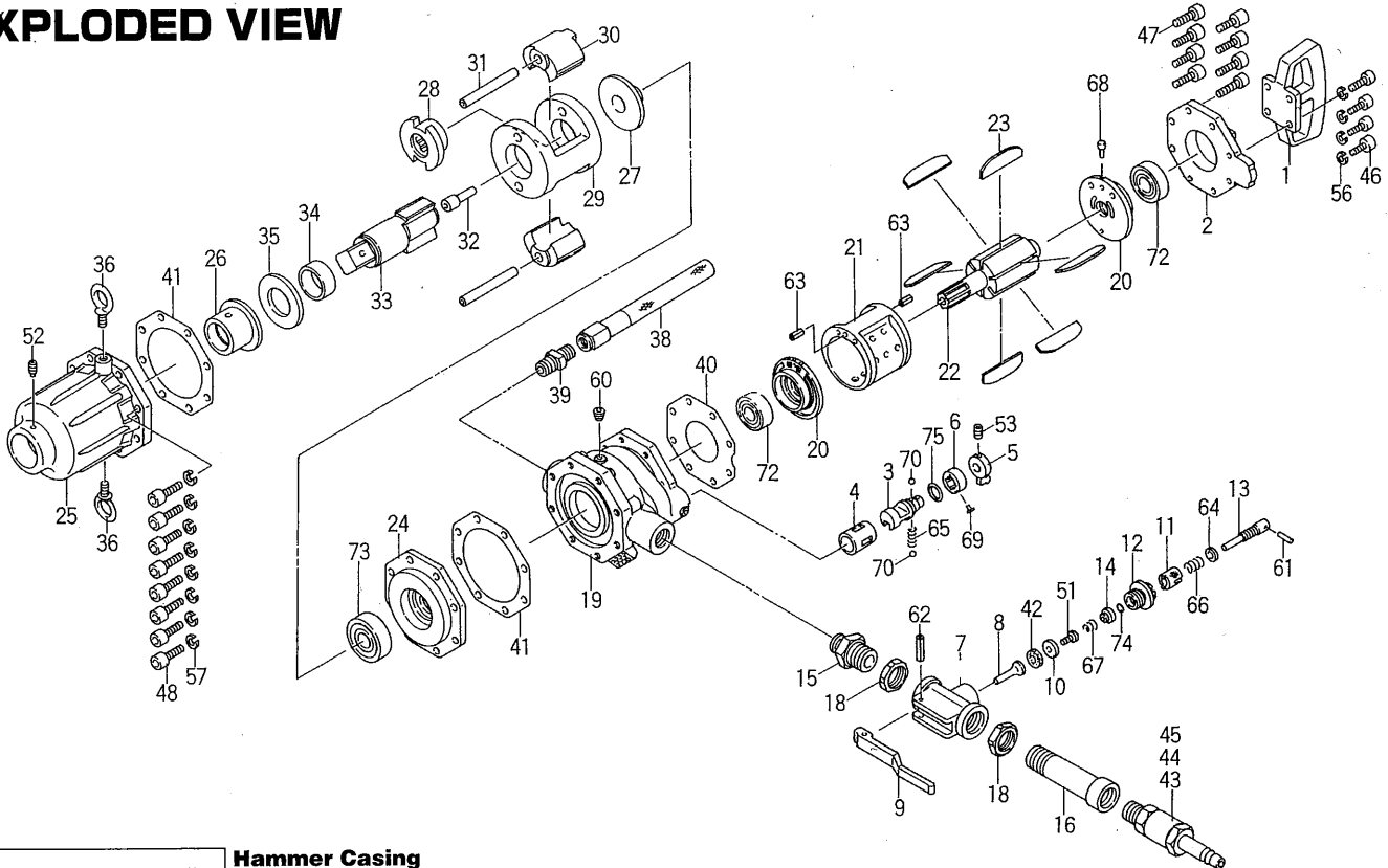
Hammer Casing Assembly Code No. 117-007-1 Components (#25, 26, 52)
