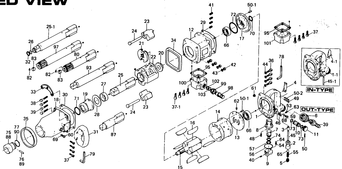
Handle Assembly (Out) Code No. 109-001-1 Components
